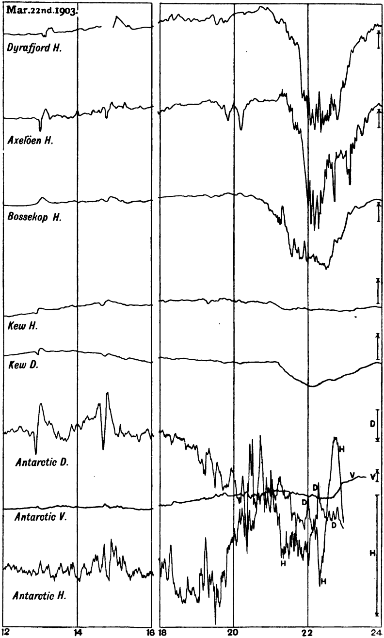
FIG. 41.—ARCTIC-KEW-ANTARCTIC CURVES.
